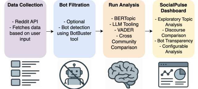
Figure 1: The SocialPulse pipeline supports rapid exploratory data analysis and sensemaking of Reddit communities; implementation details are provided in Table 2.
